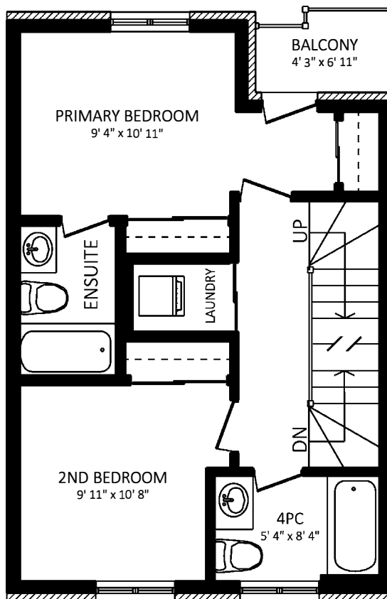
SECOND FLOOR 8' CEILING
