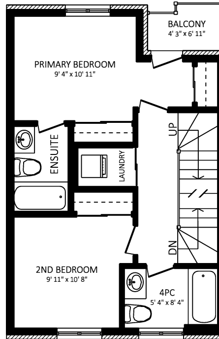
SECOND FLOOR 8' CEILING
