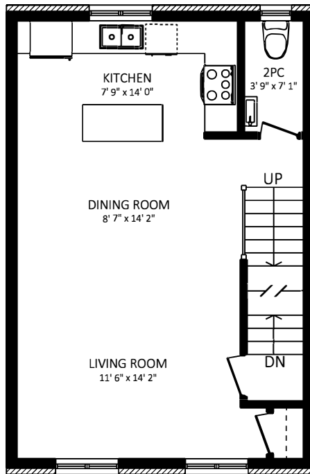
MAIN FLOOR 9' CEILING
