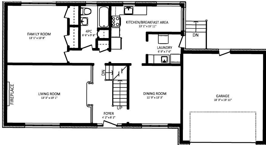
MAIN FLOOR 1190 SQUARE FEET APPROX. 8' CEILING
